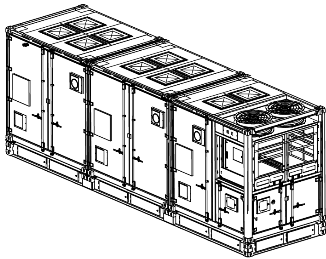
Overall Appearance
