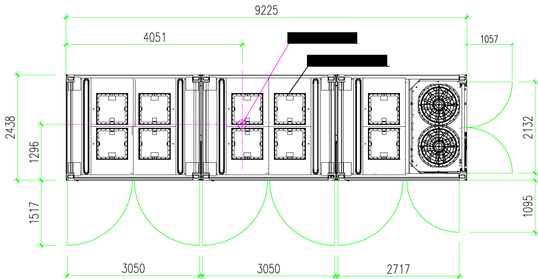
Top View
