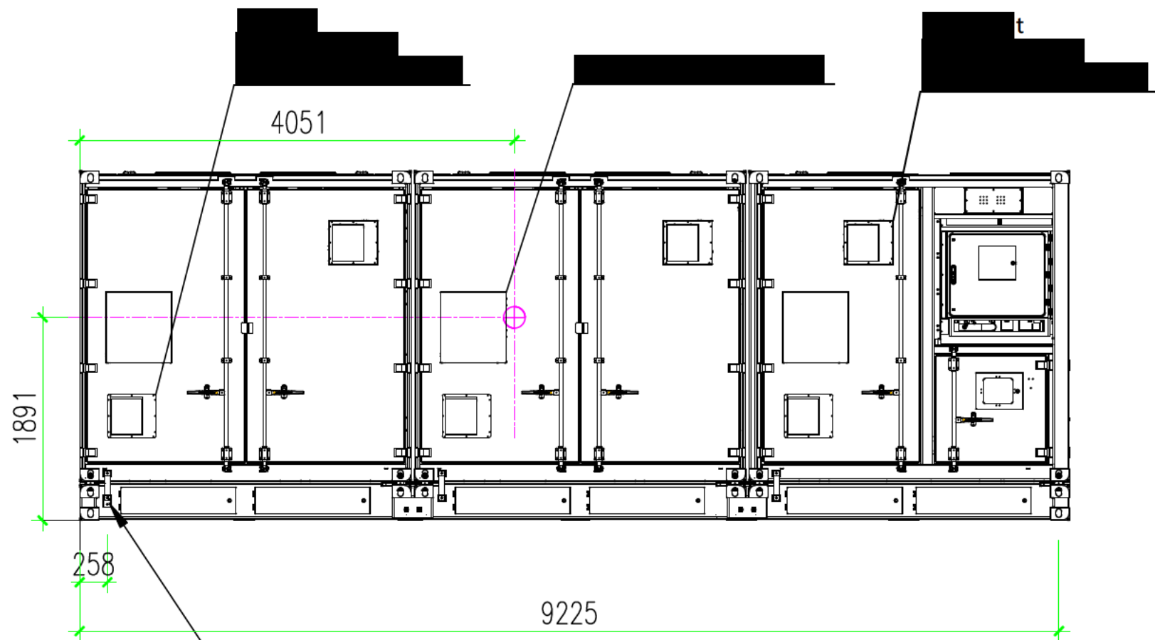
Battery Container Front View
