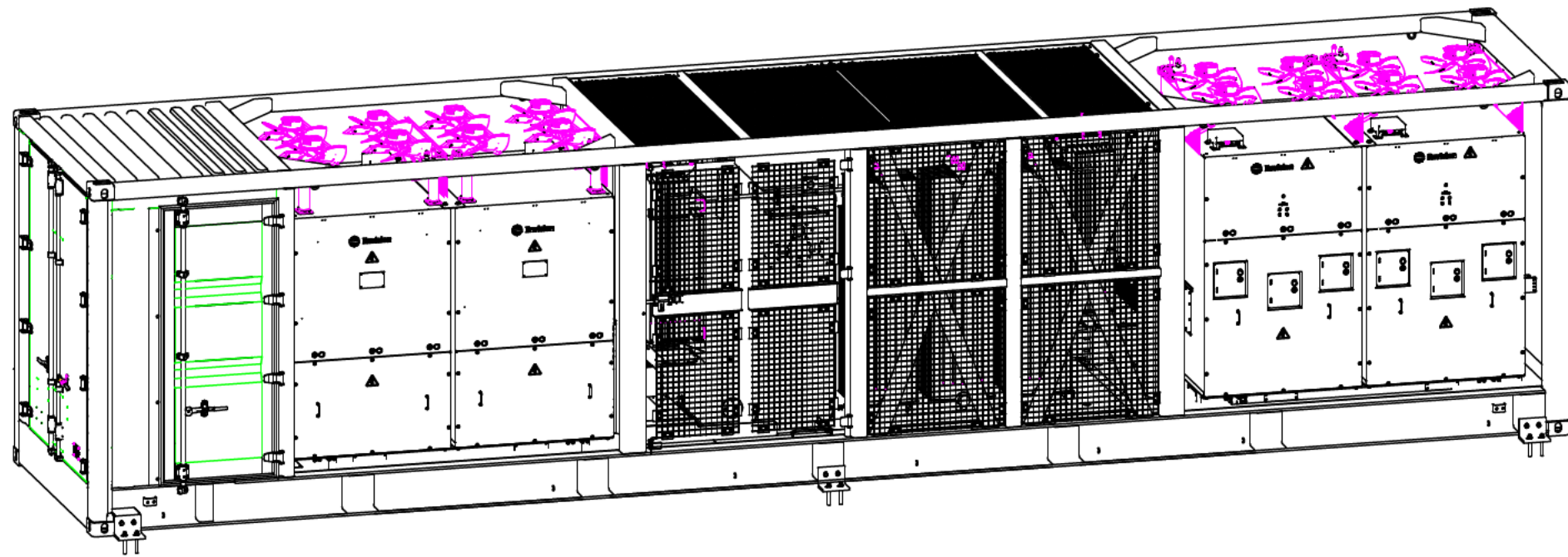
3D View
