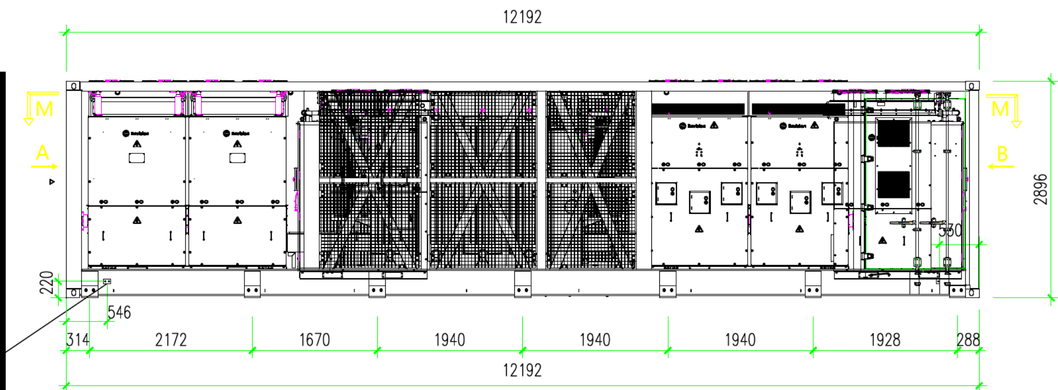
Front View
