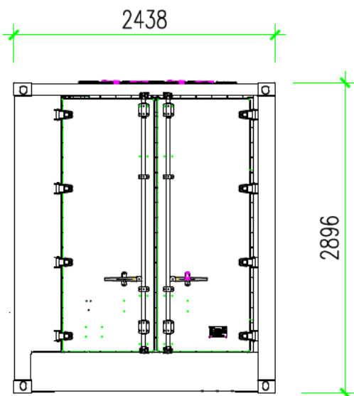
Side View B Right View
